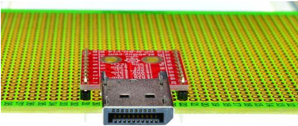
Figure 5: Solid Mounting on prototype PCB
