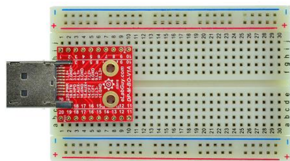
Figure 2: Example of connecting the DP-M-BO-V1A on a breadboard
